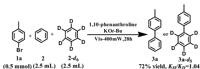
Scheme 1. KIE Experiment of the Model Reaction
