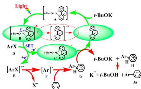
Scheme 2. Proposed Plausible Mechanism
