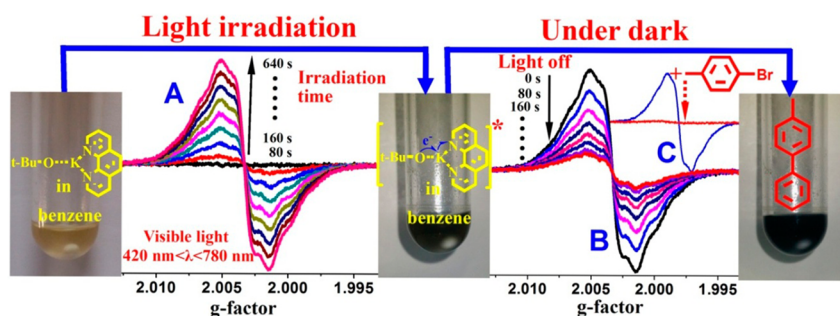
Figure 1. EPR spectra arising from the benzene solution of 1,10-phenanthroline and \text{KO}t\text{-Bu} under visible light excitation and their following decay after turning off the light (photographs showing the color changes of the mixed solution before and after light irradiation and the structure of the formed complex).
